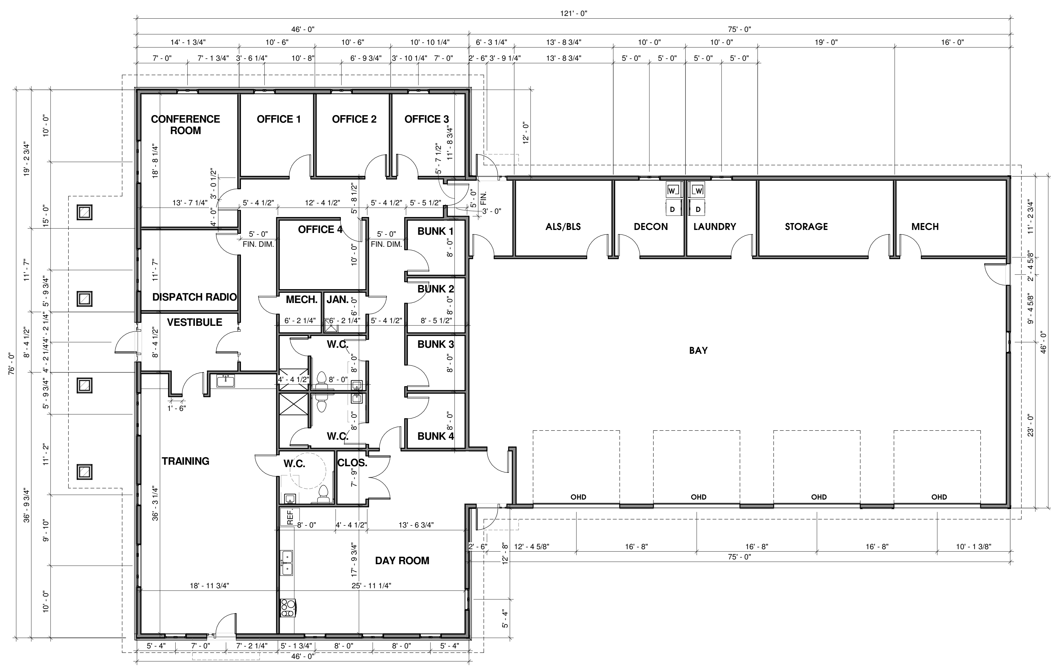
① FIRST FLOOR PLAN 0 2 4 8 16'
